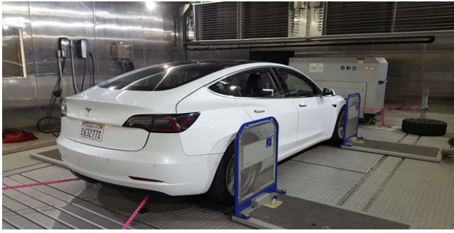
Pic of Car on Dyno - Tesla Fremont Facility
